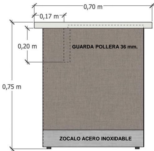
LATERAL
