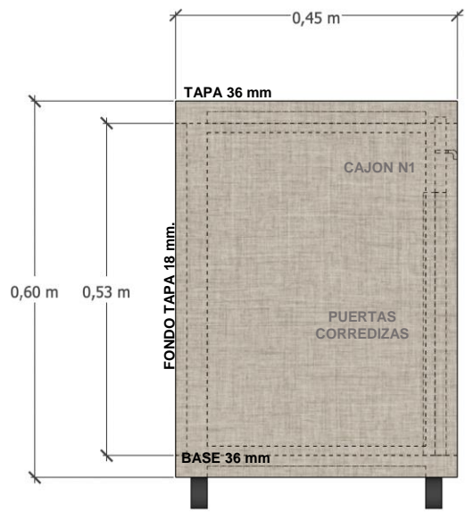
LATERAL
