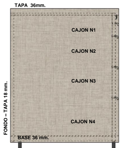
LATERAL
