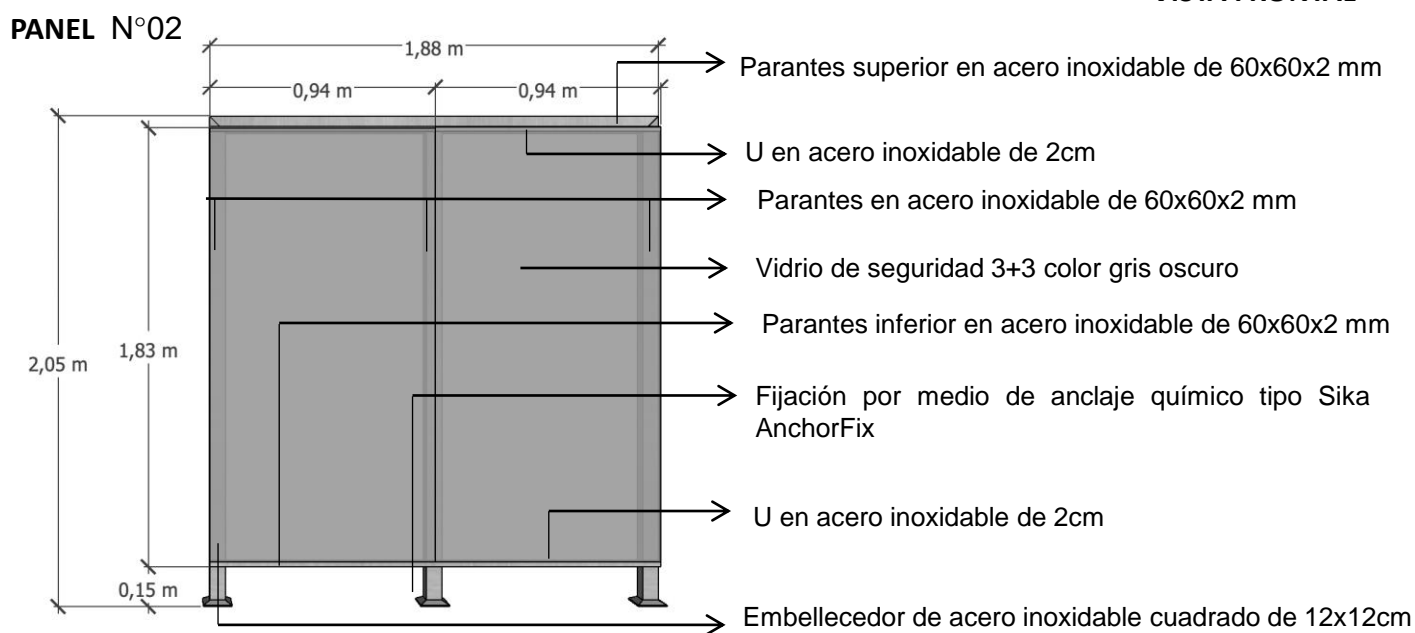
VISTA FRONTAL
